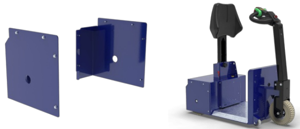
Traction wheels guard
